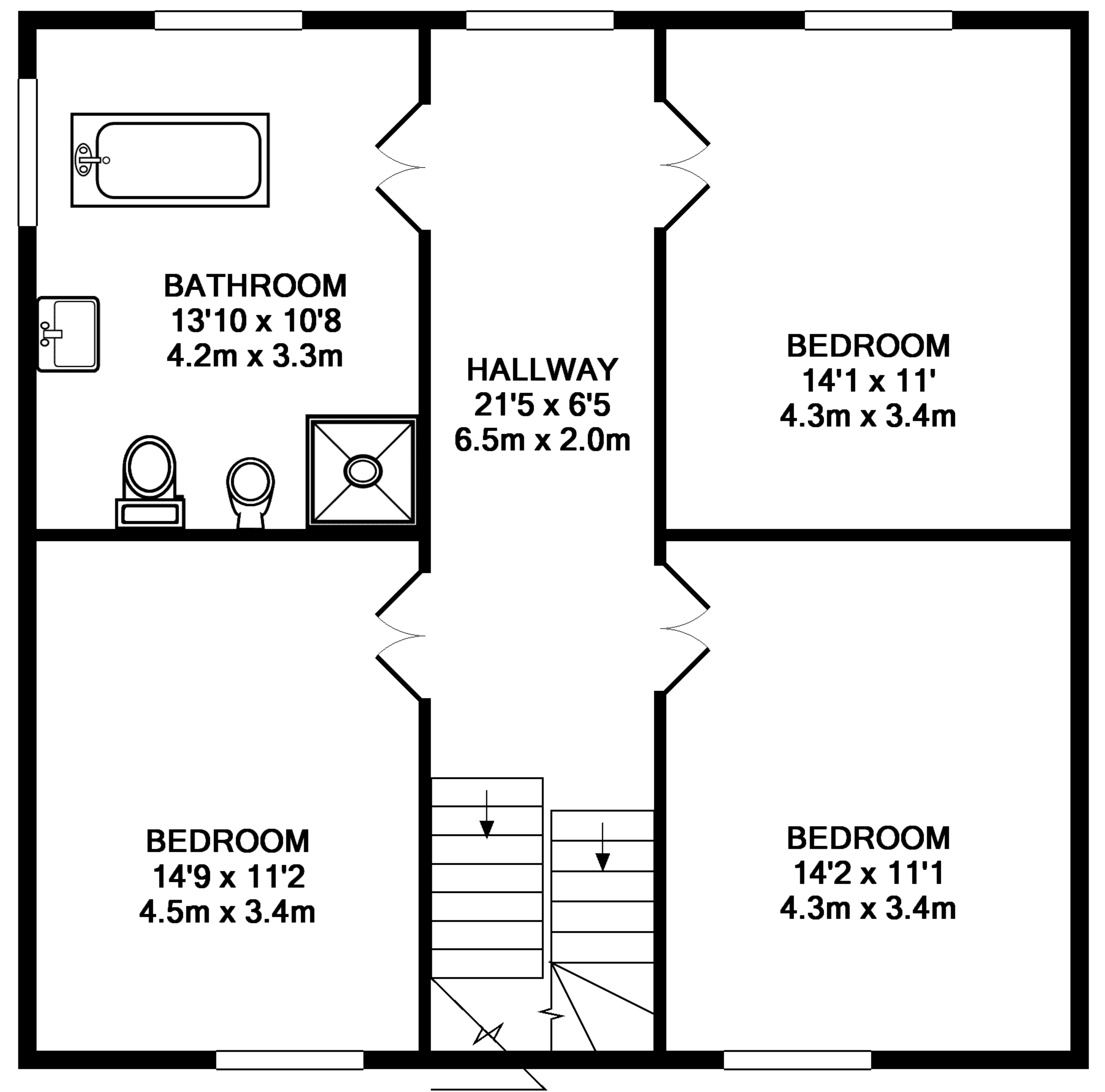
1ST FLOOR APPROX. FLOOR AREA 72.8 SQ.M. (783 SQ.FT.)
